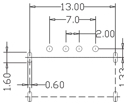
RECOMMEND PCB LAYOUT
