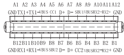
USB TYPE-C PIN ASSIGNMENTS
