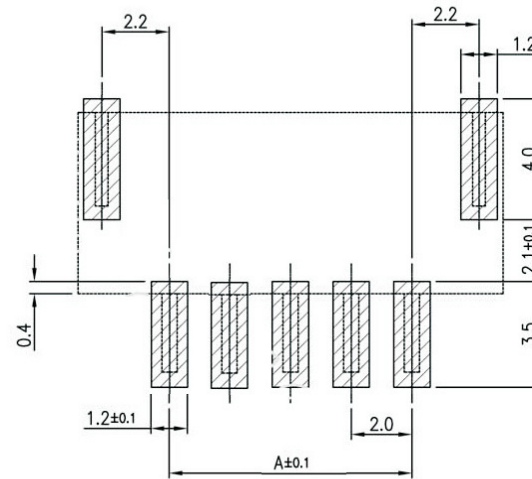
PCB PATTERN LAYOUT
