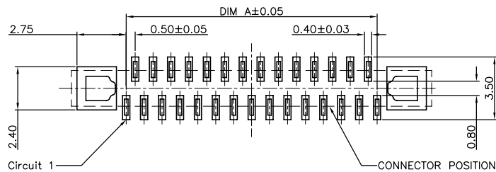
RECOMMENDED P.C.B. PATTERN LAYOUT
