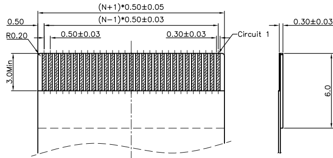
RECOMMENDED FPC/FPC DIMENSION
