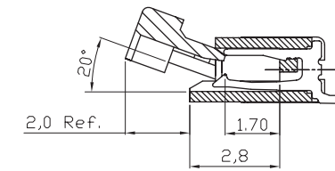
Section X-X'
