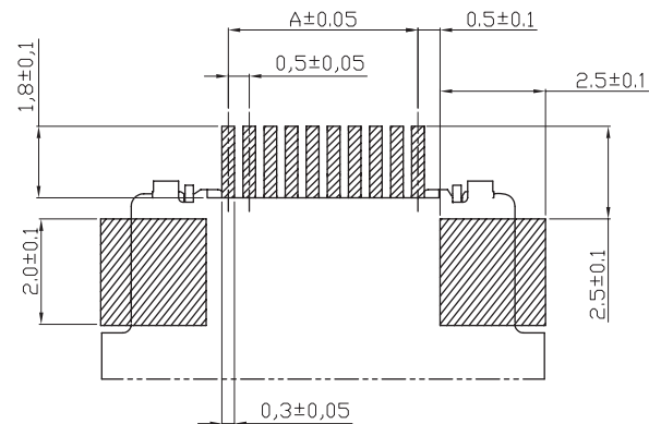
Sold Pad Pattern
