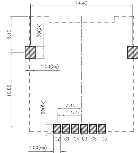
RECOMMENDED P.C. BOARD LAYOUT(TOP VIEW) GENERAL TOLERANCE:±0.05
