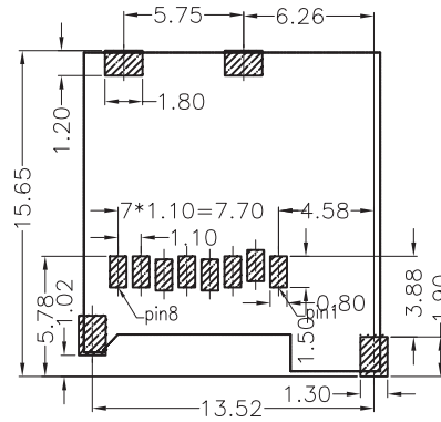
RECOMMENDED P.C.B HOLE LAYOUT COMPONENT SIDE VIEW(TOLERANCE: +/-0.05)
