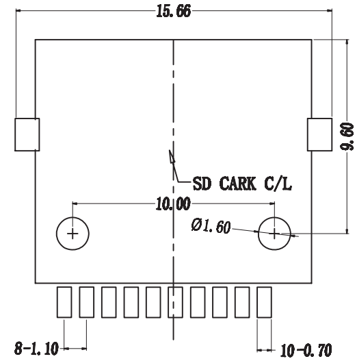
RECOMMENDED P.C.B HOLE LAYOUT COMPONENT SIDE VIEW(TOLERANCE: +/-0.05)
